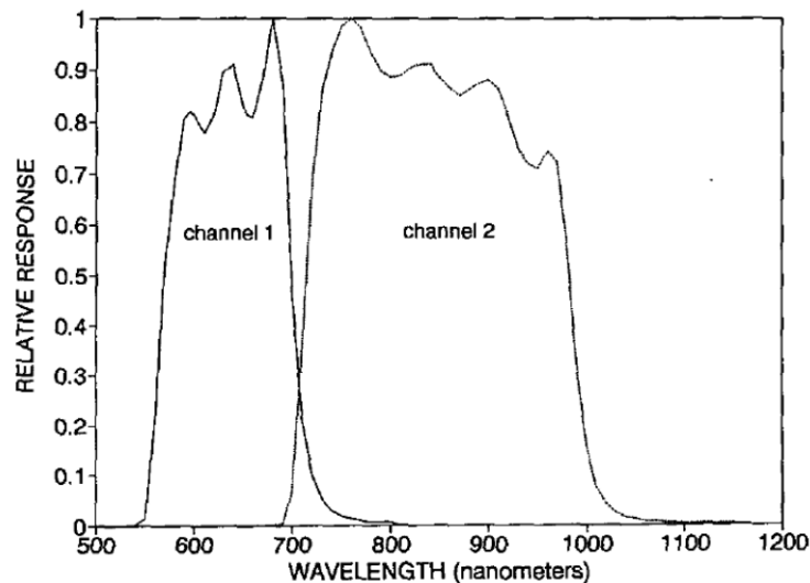
Figure 4: NOAA 9 AVHRR spectral response functions for the visible (channel 1) and the near-infrared (channel 2) detectors. Figure taken from [Hucek and Jacobowitz, 1995]
