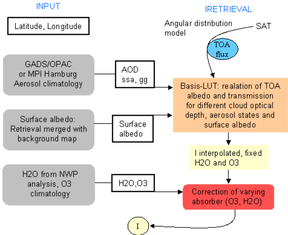
Figure 2: Diagram of the calculation of the surface solar incoming radiation under cloudy conditions. The required input data is shown on the left side of the diagram, the right part represents the calculation of the surface solar irradiance using the look-up tables for the TOA albedo. The figure is taken from [RW Mueller et al., 2009]. For the SARAH data set, an adjusted version of the GADS / OPAC aerosol climatology has been used (see text for more details).
