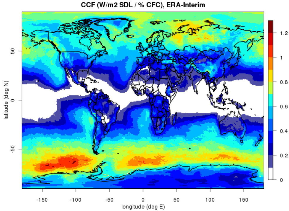
Figure 5: Temporal average of the cloud correction factor derived from the ERA-Interim data set.
