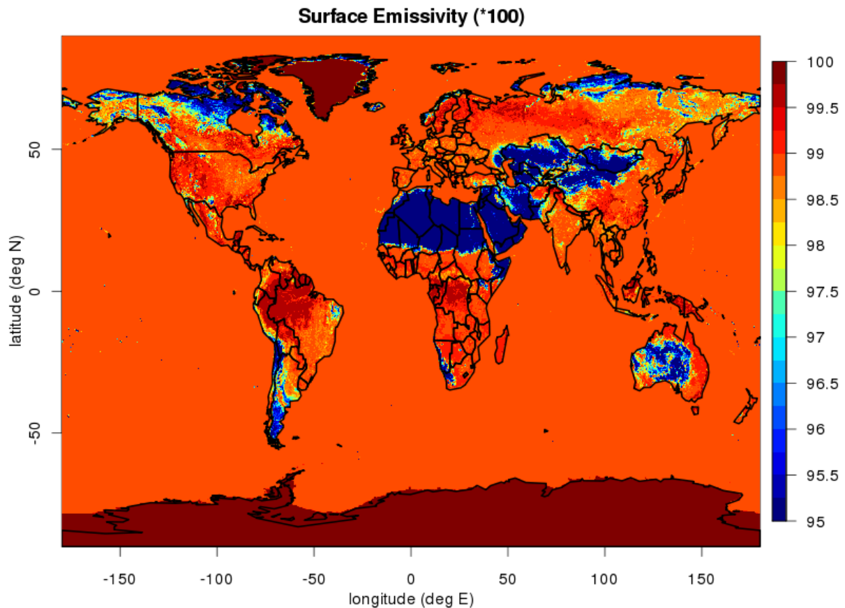
Figure 6: Surface Emissivity Map derived from land cover types.
