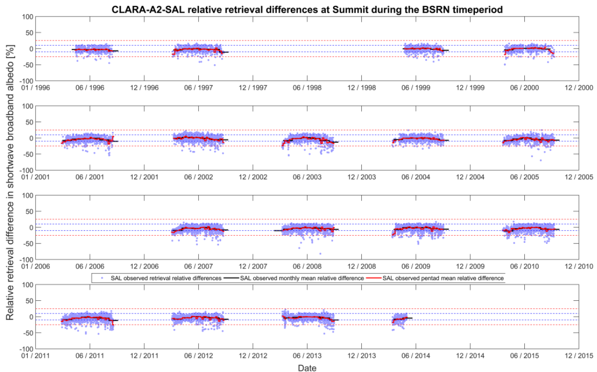
Figure 4: CLARA-A2-SAL relative retrieval difference over Summit station. Blue circles indicate retrieval differences at observed level; the black and red lines indicate the retrieval difference of the monthly and pentad mean. Red dashed line shows 25% and the blue dashed line 10% relative difference levels.
